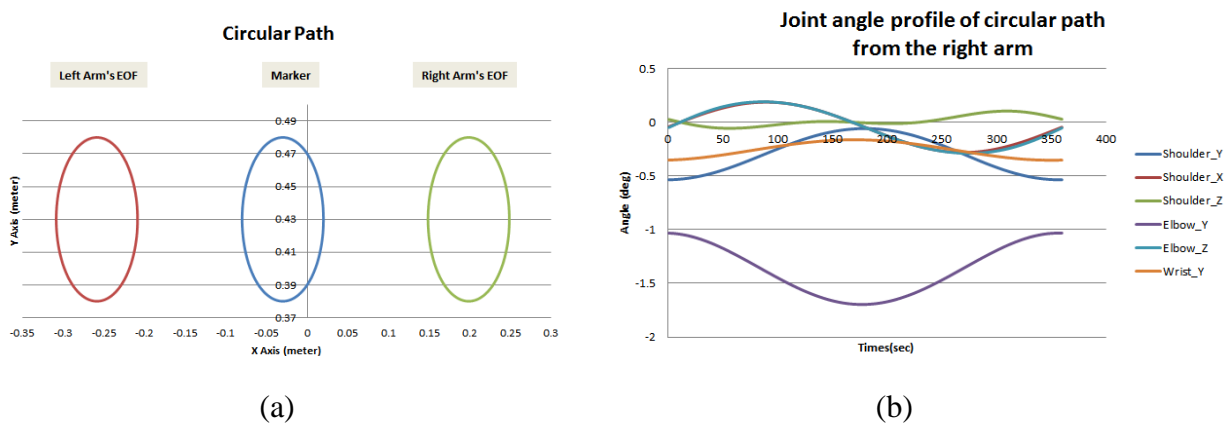
Fig. 8 The tracking result of the circular path and joint angle profile of the right arm
