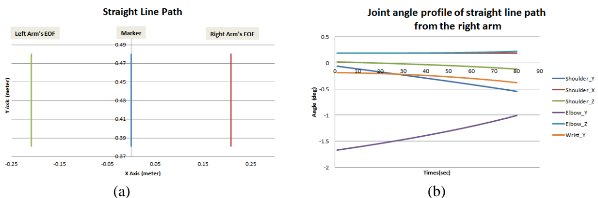
Fig. 6 The tracking result of the straight line path and joint angle profile of the right arm
