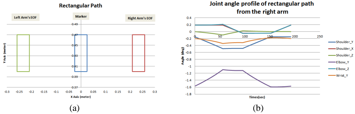
Fig. 7 The tracking result of the rectangular path and joint angle profile of the right arm
