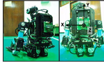
Fig. 7 The experimental humanoid robot – KM4 and 6-DOF IMU on his back
